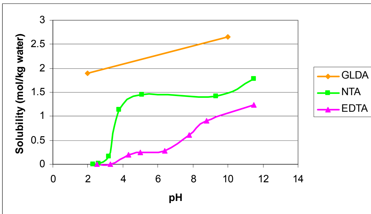
Figure 3: Solubility of chelating agents in water at various pH levels
