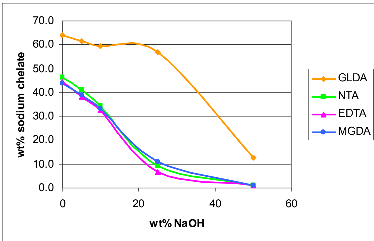
Figure 4: Solubility of chelating agents in concentrated sodium hydroxide solution.
