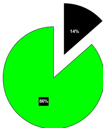
Figure 2: GLDA-Na4 fossil & green character
